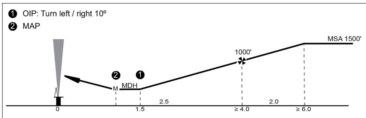
Figure 2 — Vertical profile
