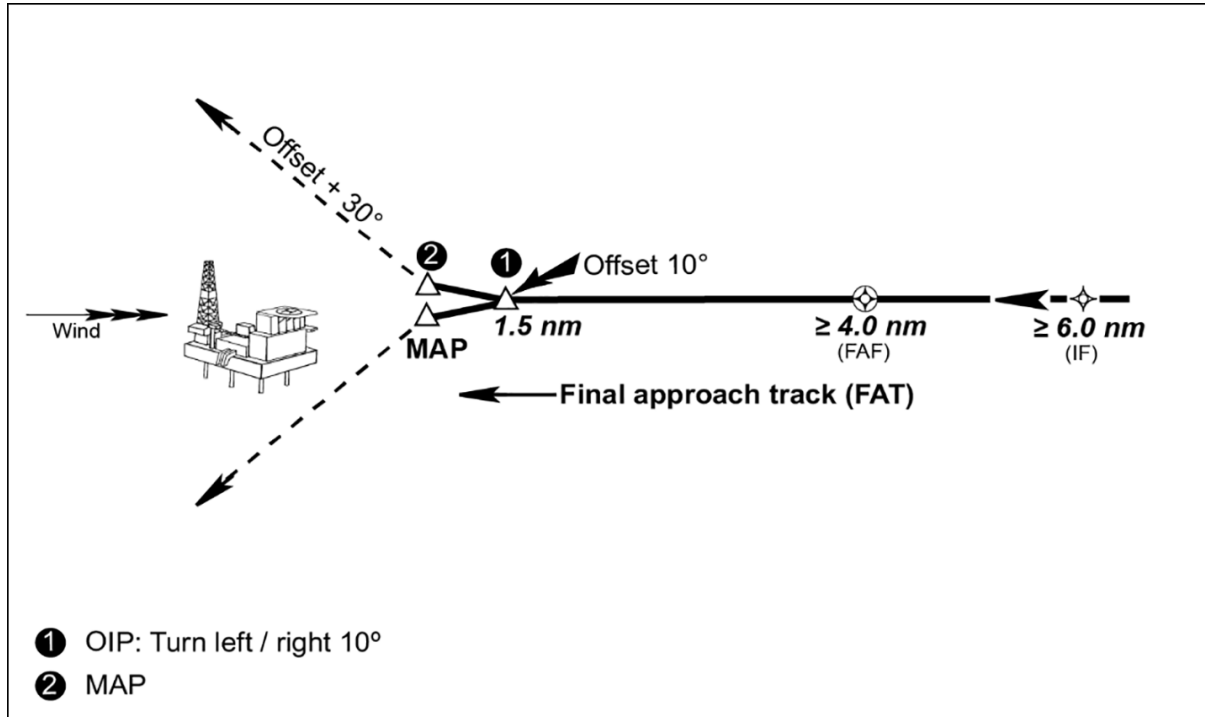
Figure 1 — Horizontal profile
